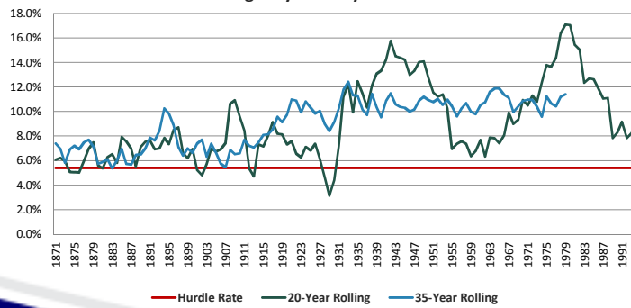
Rolling Historical Returns Over 20- & 35-Year Time Horizons vs. 5.4% Longevity Annuity Hurdle Rate
